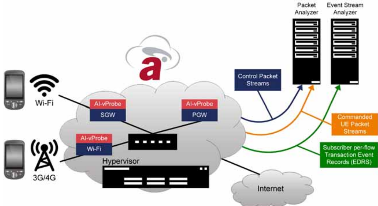
Figure 1-1 AI-vProbe Network Deployment
